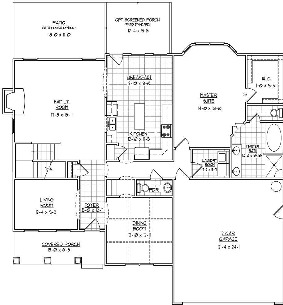
FIRST FLOOR
