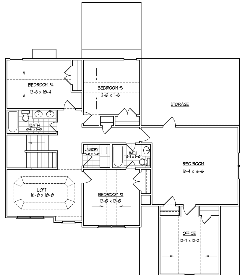
SECOND FLOOR
